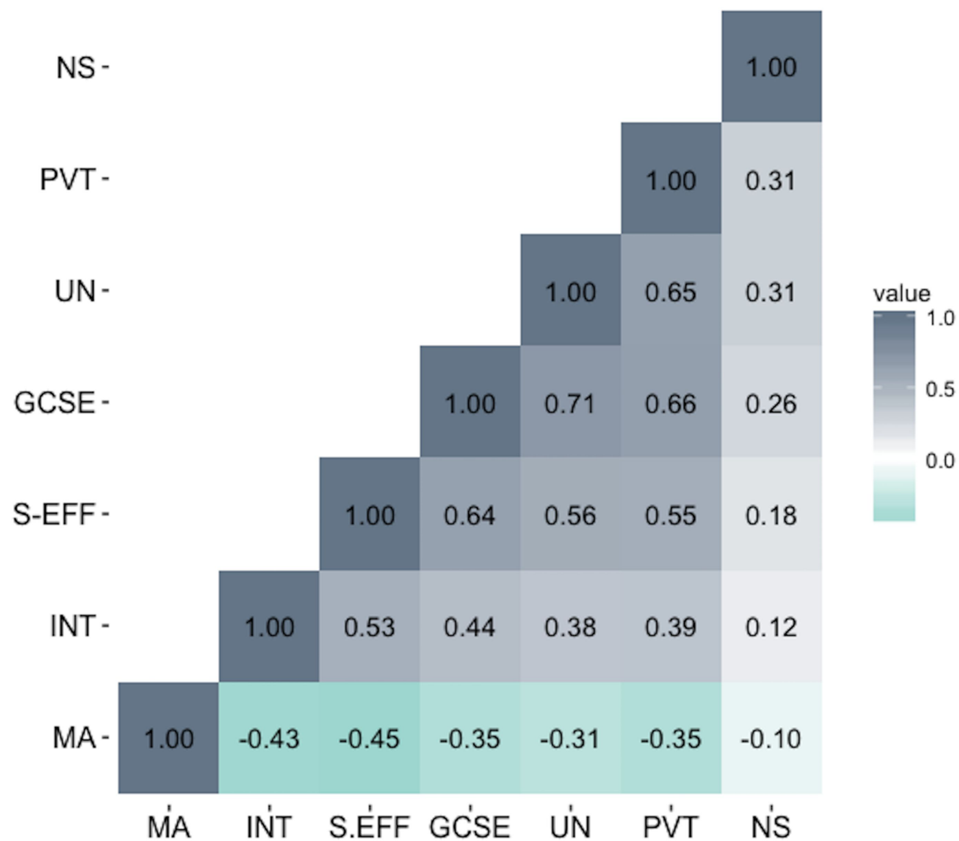
Phenotypic correlations
