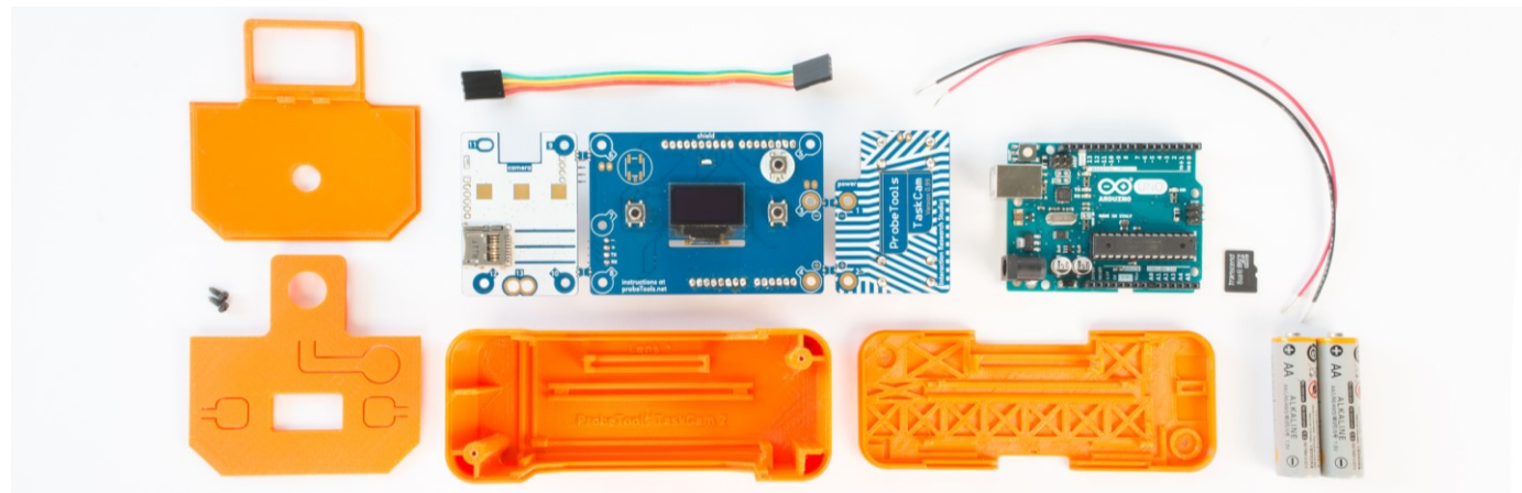
Figure 2. 3D TaskCam with hardware components: custom PCB, Arduino Uno, SD card and batteries. © 2018 Interaction Research Studio
