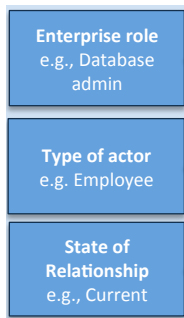
Fig. 4. Actor elements
