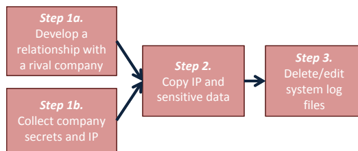
Fig. 6. Attack Steps
