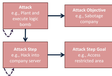
Fig. 5. Attack elements
